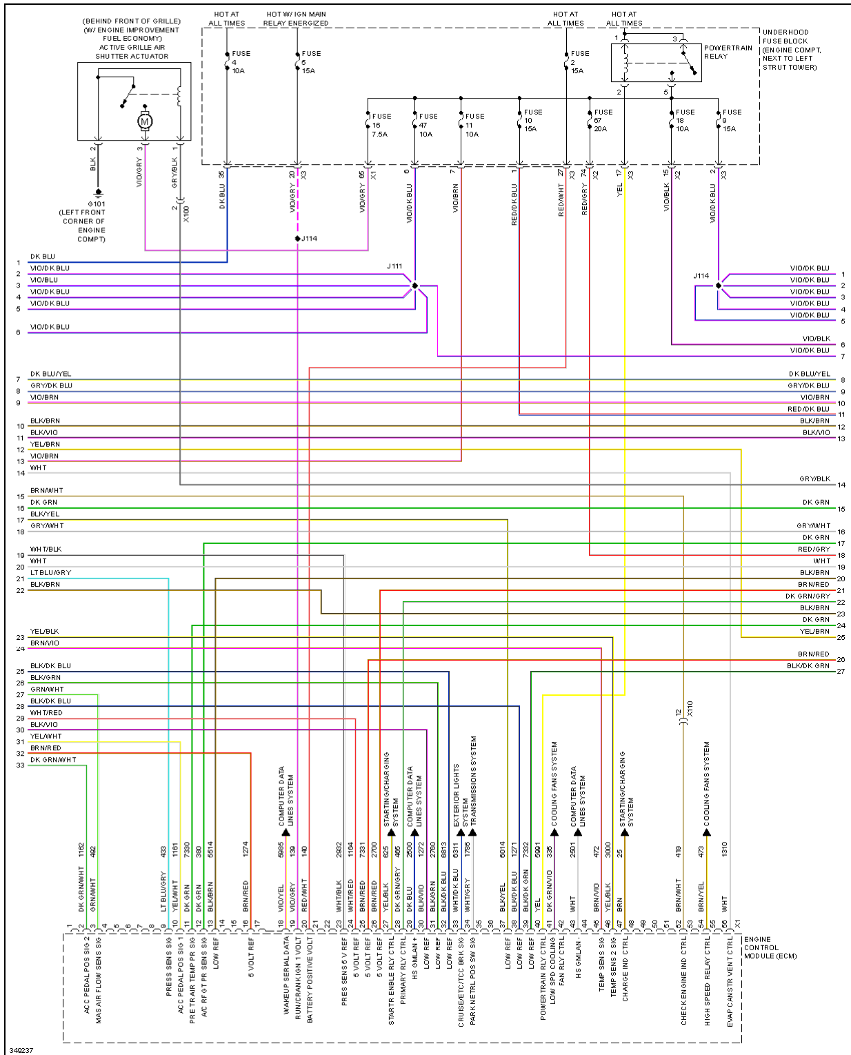
Fig. 20: 1.4L VIN 9, Engine Performance Circuit (3 of 6)
