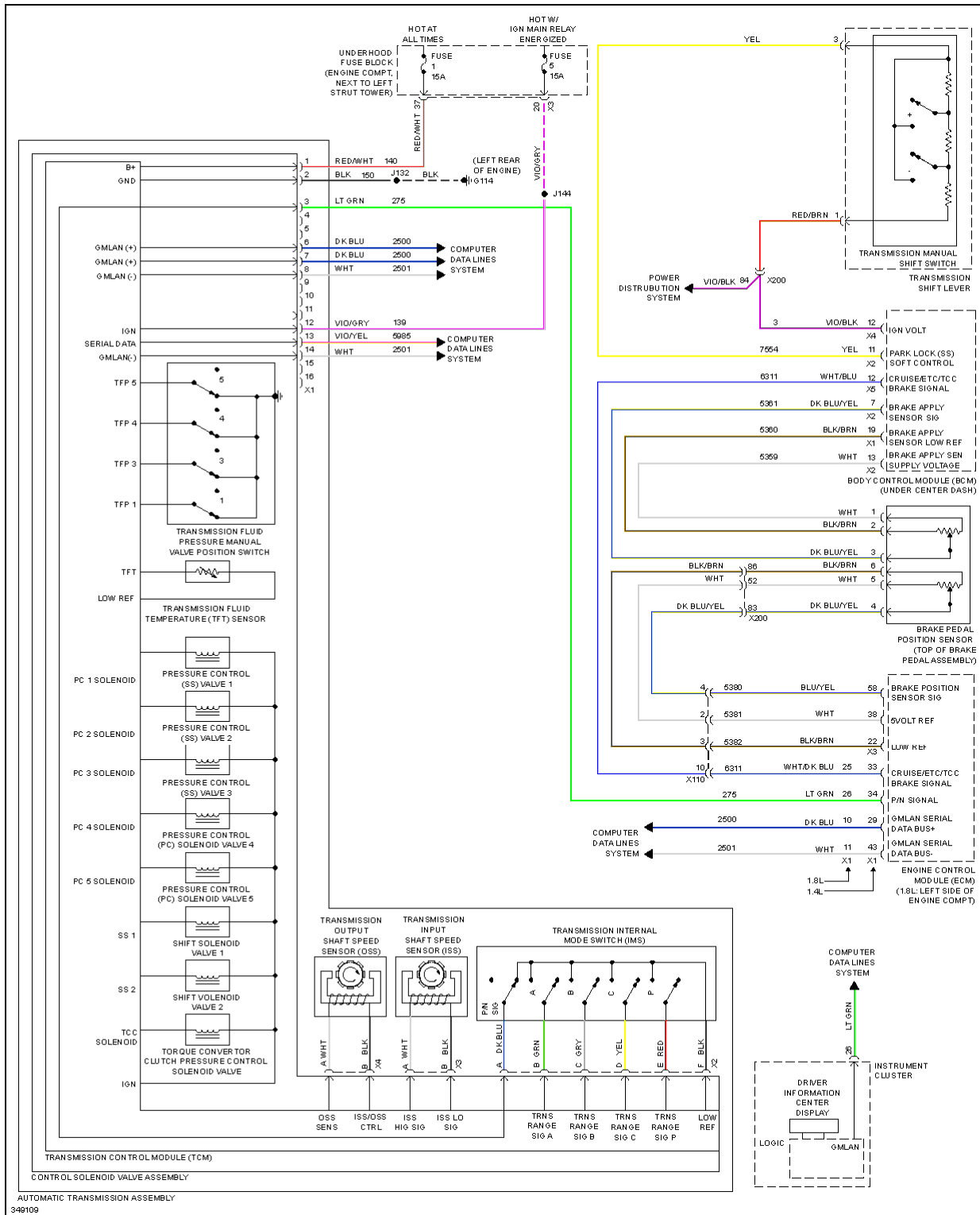
Fig. 73: Transmission Circuit
