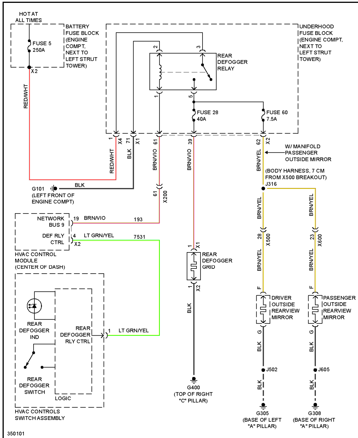
Fig. 16: Defoggers Circuit
