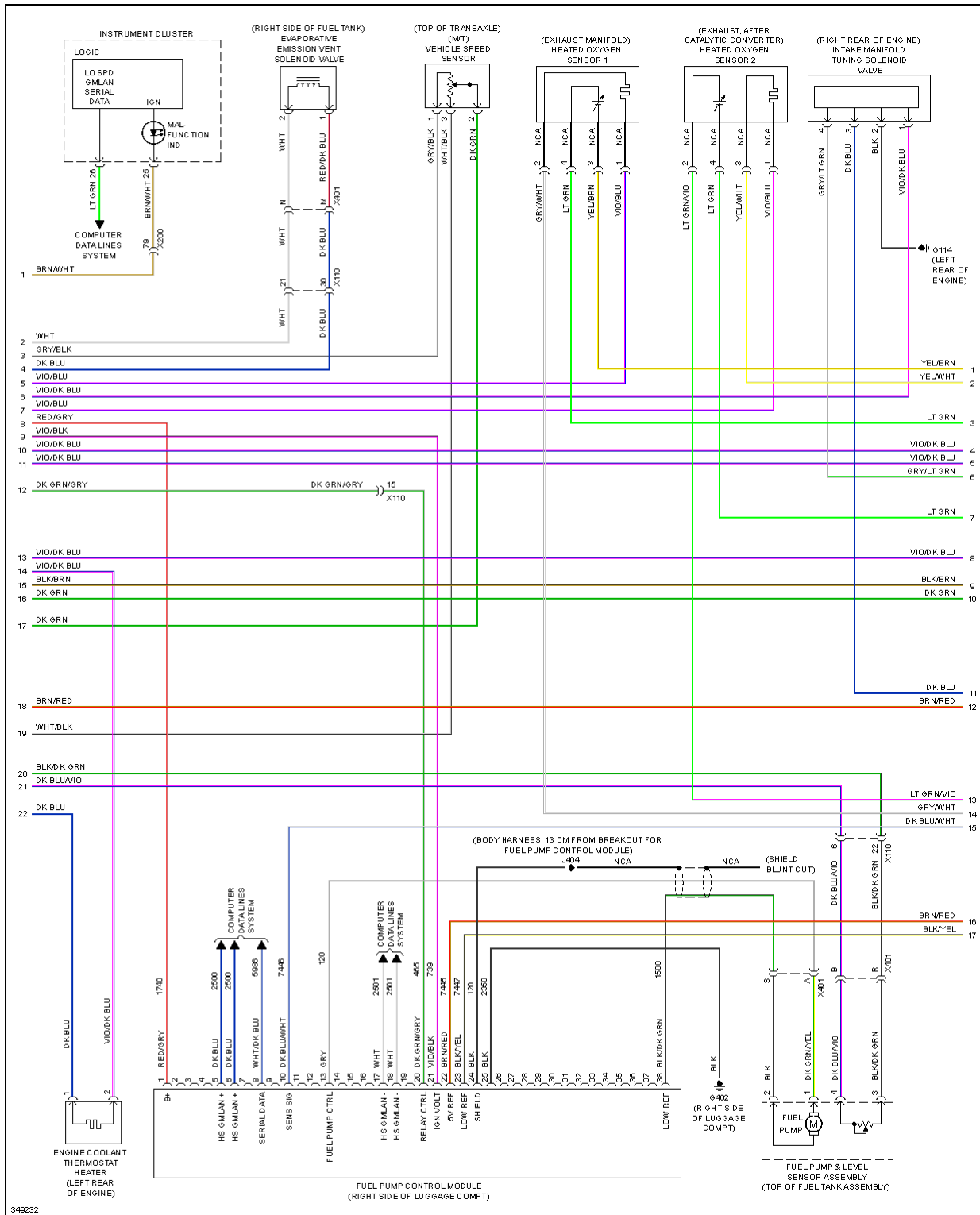
Fig. 25: 1.8L VIN H, Engine Performance Circuit (2 of 4)
