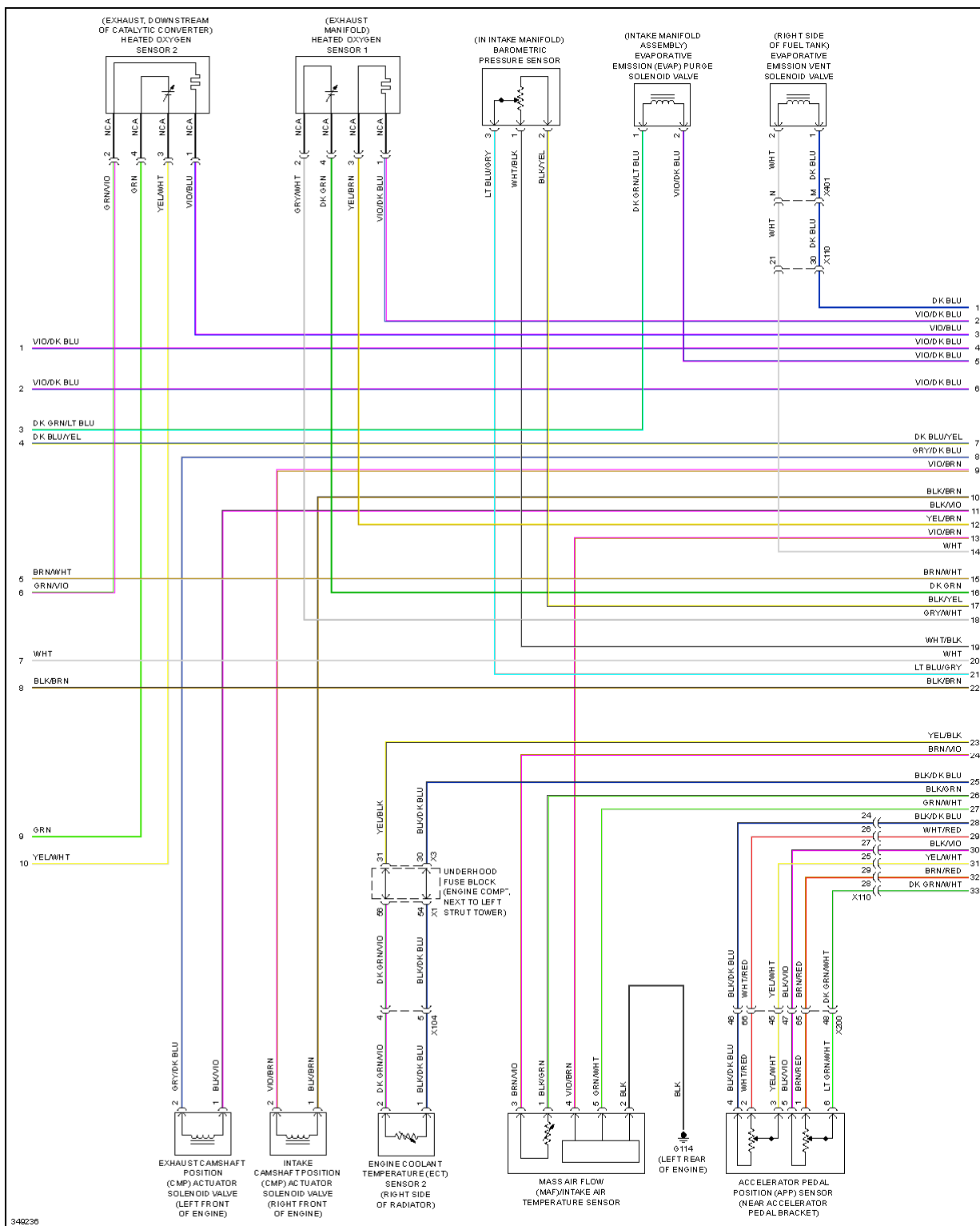
Fig. 19: 1.4L VIN 9, Engine Performance Circuit (2 of 6)
