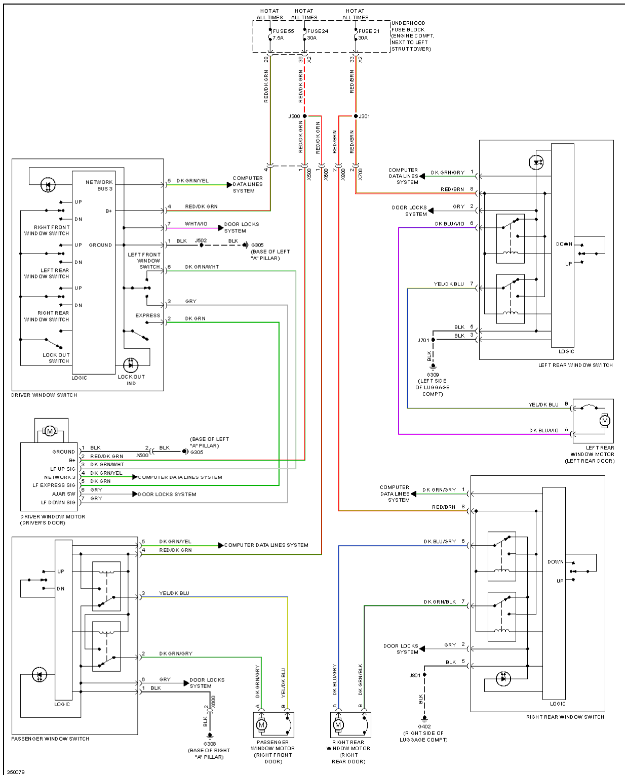
Fig. 58: Power Windows Circuit, W/ Express Up/Down
