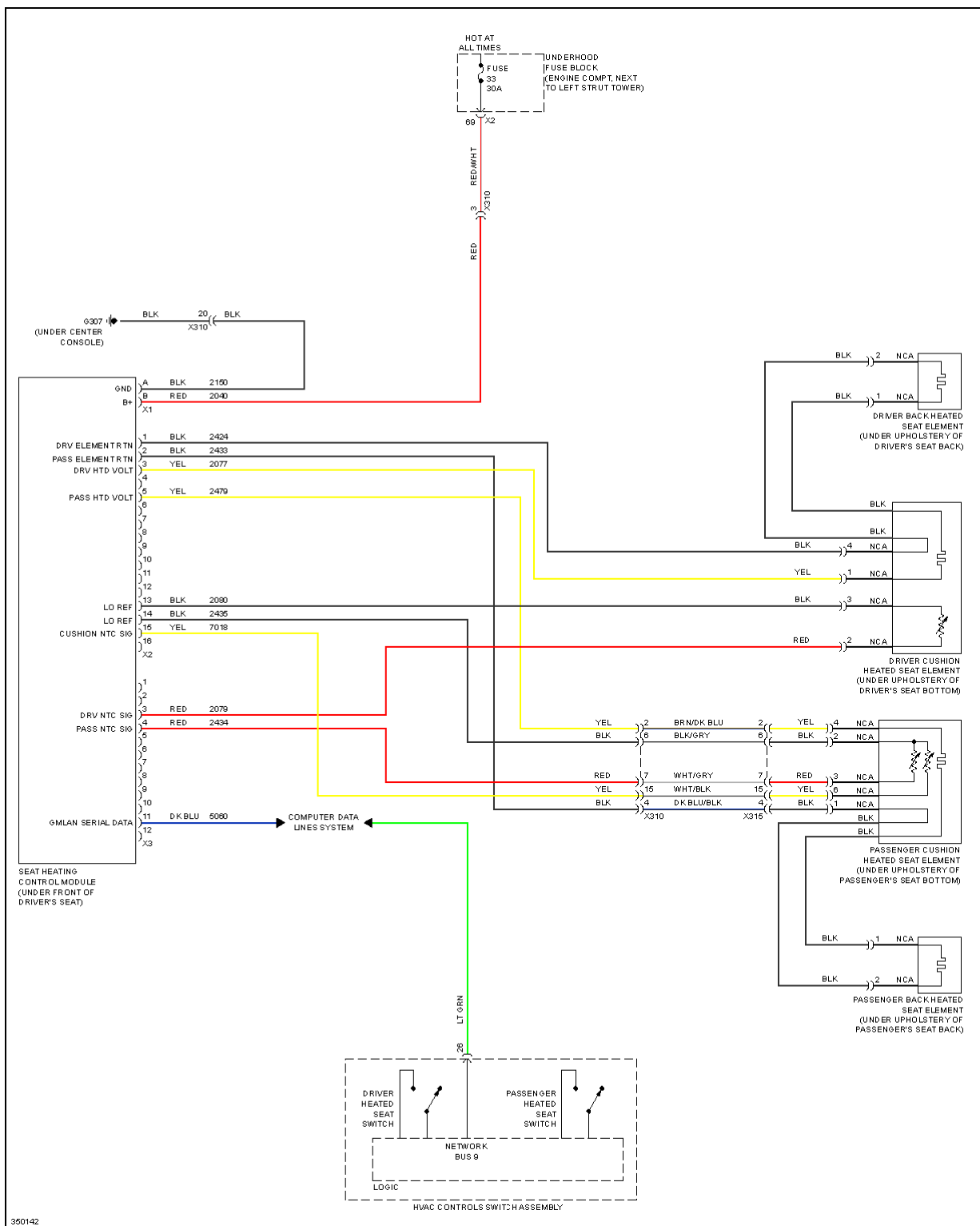
Fig. 56: Heated Seats Circuit
