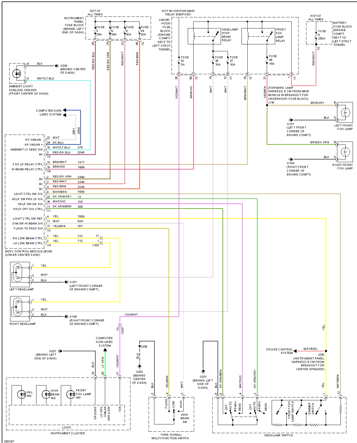
Fig. 34: Headlights Circuit
