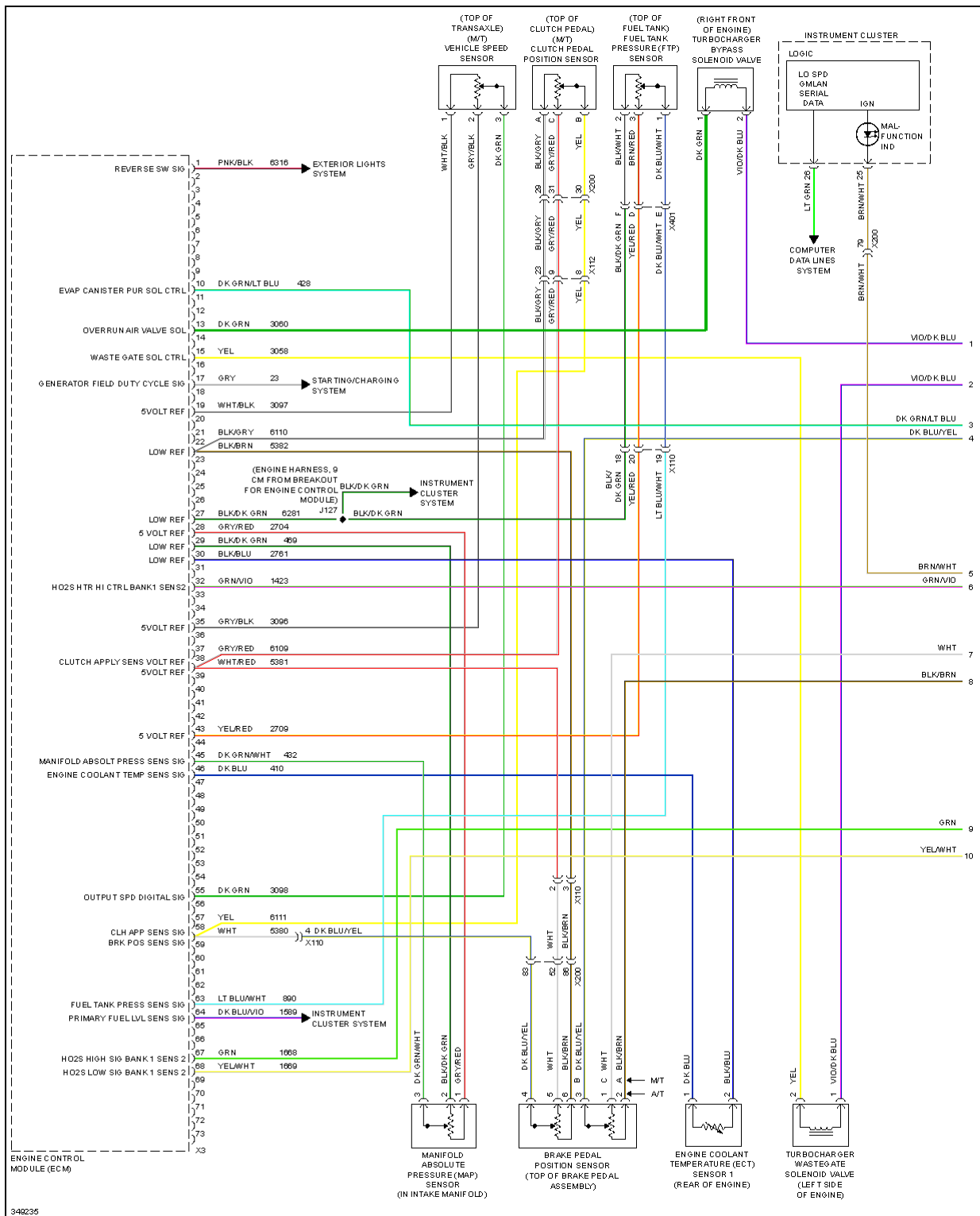
Fig. 18: 1.4L VIN 9, Engine Performance Circuit (1 of 6)
