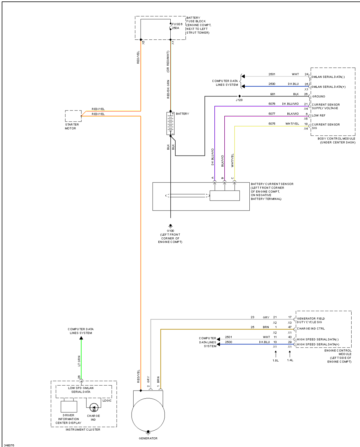
Fig. 69: Charging Circuit
